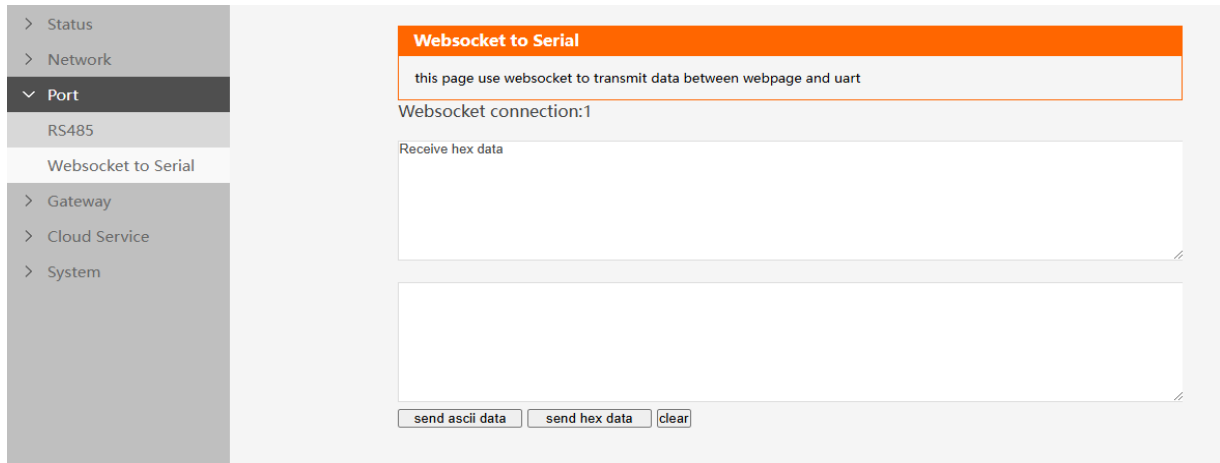
Fig 6 Send and receive data using webpage
